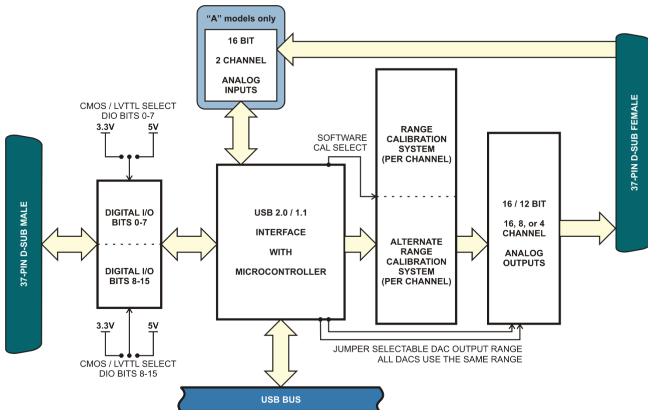
Figure 1-1: Block Diagram
