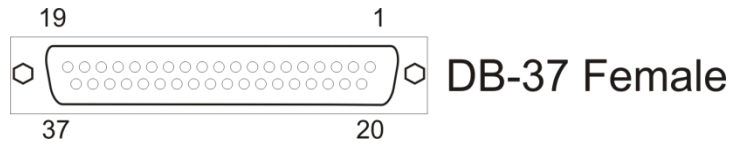
Figure 6-1: J1 DB37F Connector Pin Arrangement
